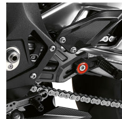
2 HP rider footrest system, left
